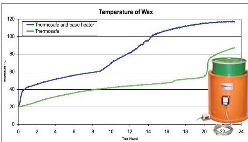
Temperature measured at the base of drum
